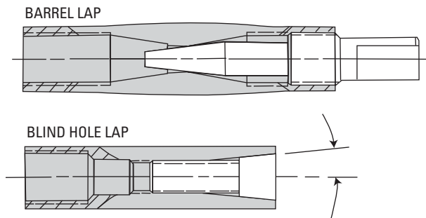
BACK TAPER TO INSURE DIAMETRAL CONTACT AT FRONT END OF LAP
